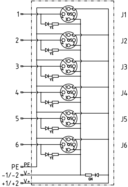
WIRING DIAGRAM
